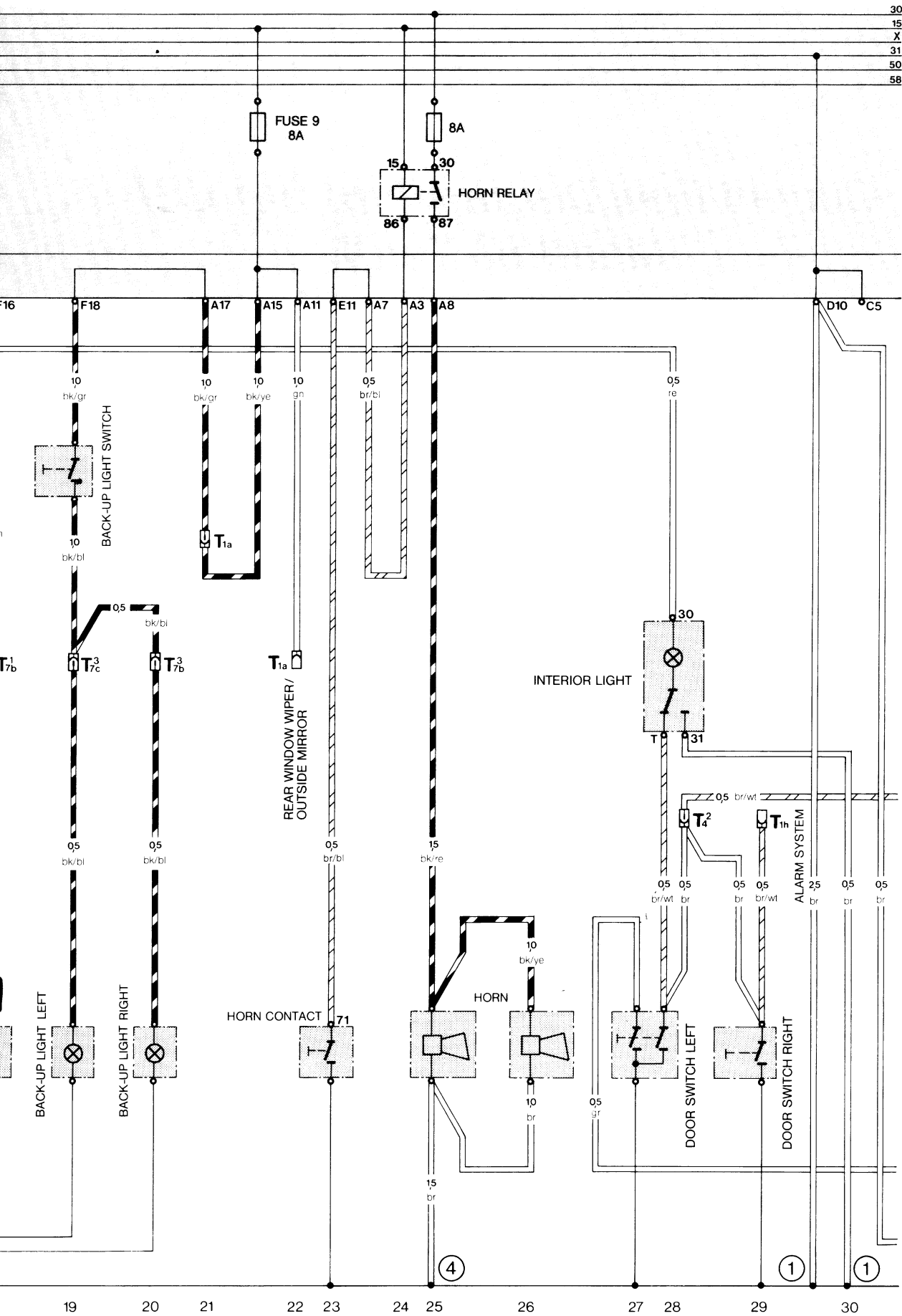
SIGNAL, BACK-UP LIGHT | HORN | INTERIOR LIGHT
