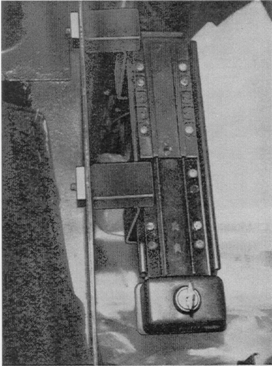
The universal holder is mounted to the fastening brackets with 4 M 4 x 10 screws.
