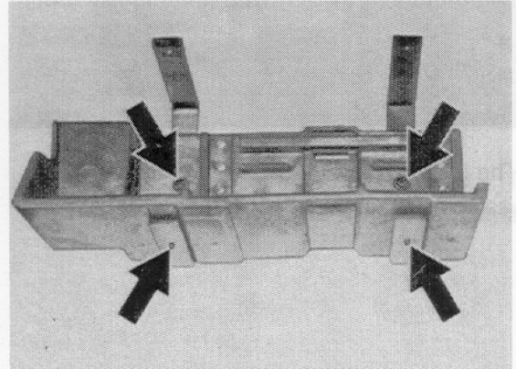
The universal holder is mounted on the 2 fastening brackets with 4 M 6 x 18 screws.
